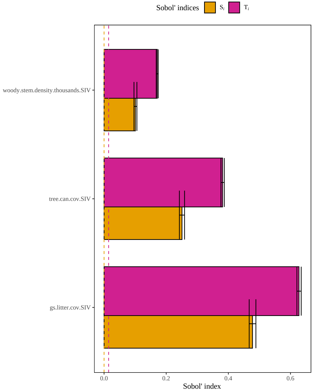
Figure 3. Results of a sensitivity analysis for the brownthrasher model based on the original multiplicative model outlined in Cade (1986). Dashed lines represent baseline numerical approximation error for S_i and T_i ( i.e. , dummy variables).
