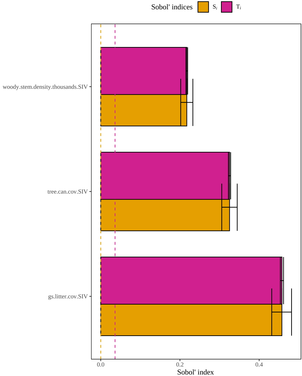
Figure 4. Results of a sensitivity analysis for the brownthrasher model based on an arithmetic mean structure. Dashed lines represent baseline numerical approximation error for S_i and T_i ( i.e. , dummy variables).
