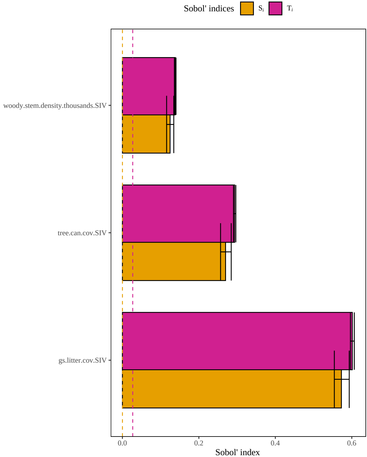
Figure 5. Results of a sensitivity analysis for the brownthraasher model based on a geometric mean structure. Dashed lines represent baseline numerical approximation error for S_i and T_i ( i.e. , dummy variables).
